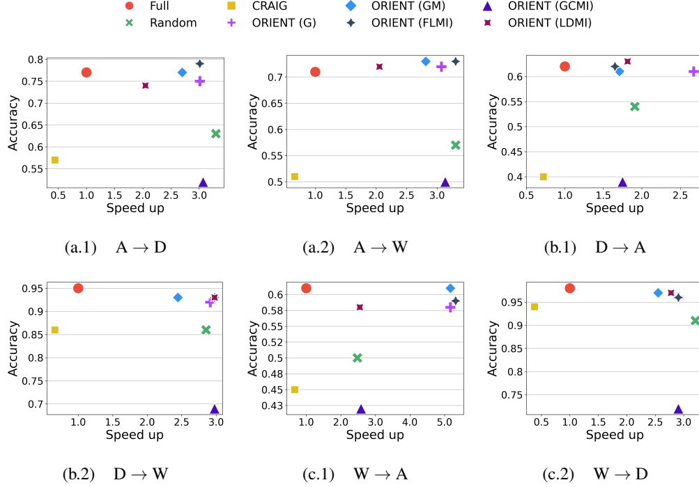
Figure 2: Speed up vs prediction accuracy on three domains of Office31 dataset: Amazon (A), DSLR (D), and Webcam (W). X-axis represents the speed up by the model, i.e. the ratio of the time taken to train on complete source dataset (Full) to the time taken by the model. Y-axis represents the prediction accuracy of the model on the target domain.
