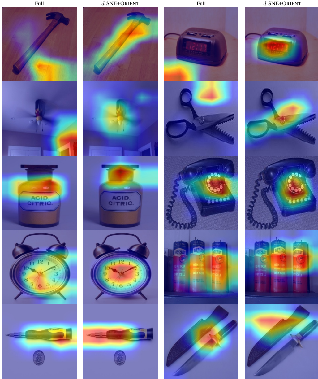
Figure 6: GradCam [45] activation maps of the models learned using d -SNE + Full and d -SNE + ORIENT (FLMI) on the Office-Home dataset with "Product" as the source domain and "Real World" as the target domain. As evidenced by class activation maps, the ORIENT framework enabled the model to learn more effective class discriminative features than Full data training consistently.
