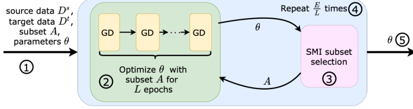
Figure 1: Illustration of ORIENT framework. (1) Given the target data D^t and source data D^s , a subset A \subseteq D^s and model parameters \theta are randomly initialized. (2) Model parameters \theta are optimized for L epochs on the subset A with any gradient descent (GD) based method. (3) Subset A is updated using the SMI measure and current model parameters \theta after every L^{th} epoch. (4) Model is trained for E epochs, with subset selection after every L interval. (5) The final model parameters are returned after E epochs.
